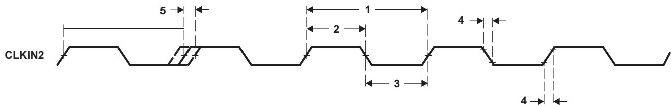
Figure 7-33. CLKIN2 Timing
