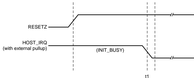
Figure 2. HOST_IRQ Timing Diagram
