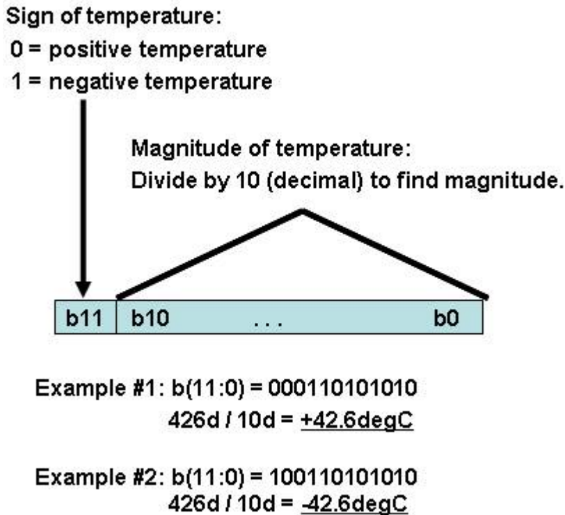
Figure 15. Bit Order and Definition for System Temperature
