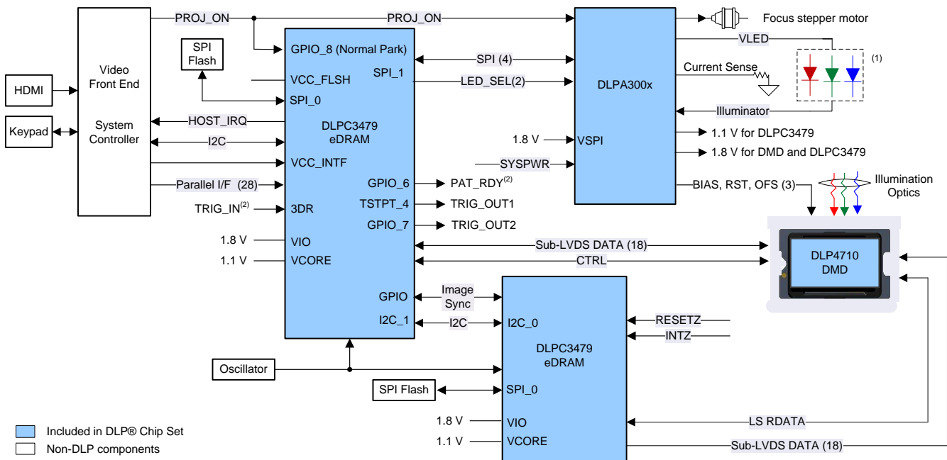
Figure 1. DLPC3479 System Block Diagram
