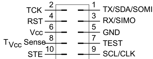
Figure 7. Pinout of the BSL Connector (Target Side)
