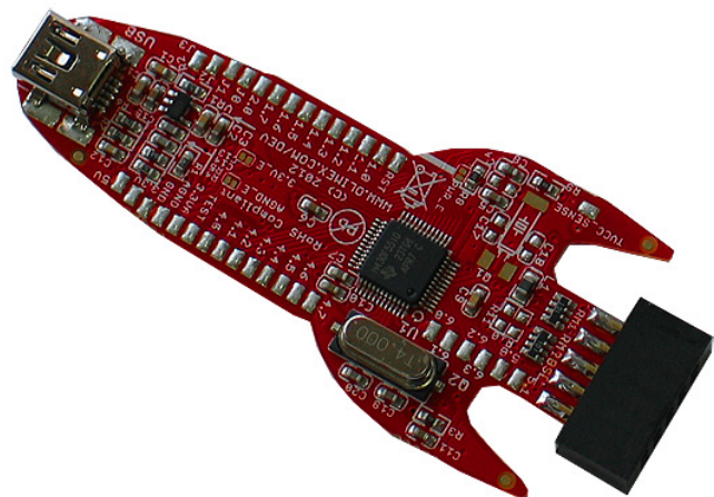
Figure 2. MSP-BSL (Bottom View)
