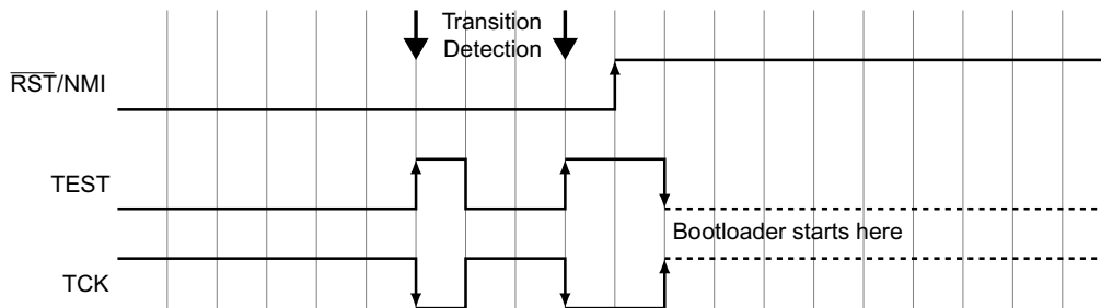
Figure 3. BSL Entry Sequence With Shared and Dedicated JTAG Pins
