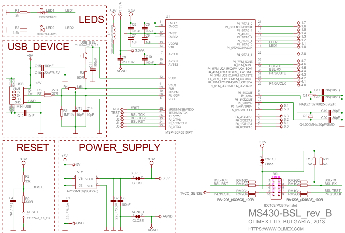
Figure 6. Schematic of the MSP-BSL
