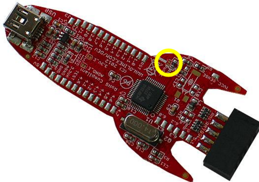
Figure 8. Cuttable Power Supply Trace (PWR_E)
