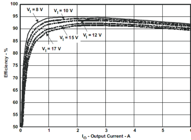
Figure 1. TPS54620EVM-374 Efficiency
