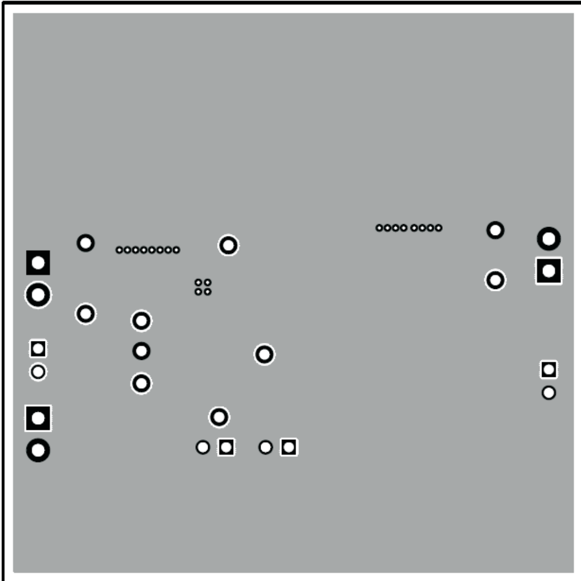
Figure 13. TPS54620EVM-374 Layout 2
