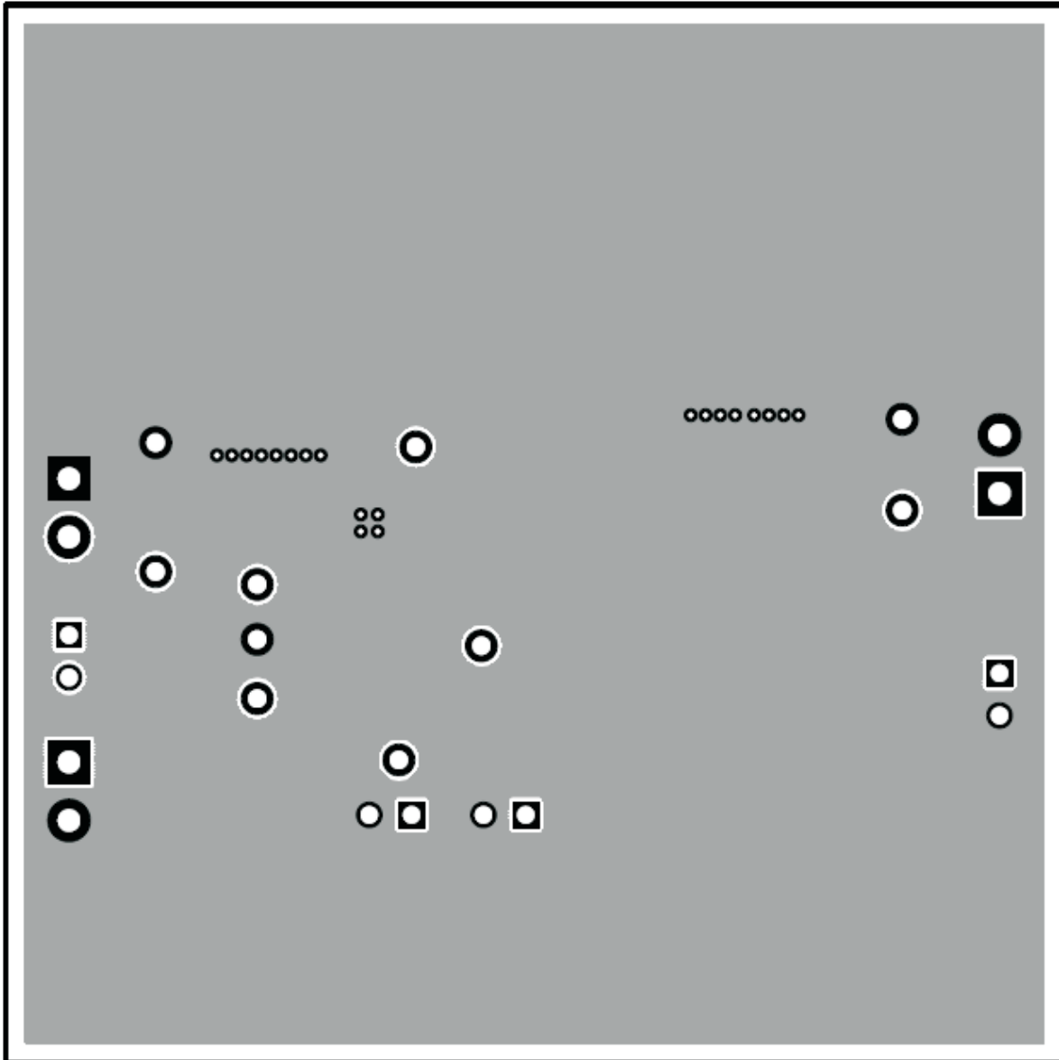
Figure 14. TPS54620EVM-374 Layout 3
