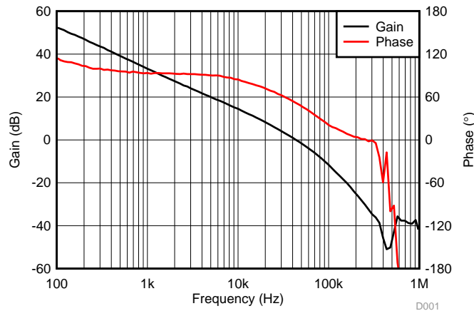
Figure 6. TPS54620EVM-374 Loop Response
