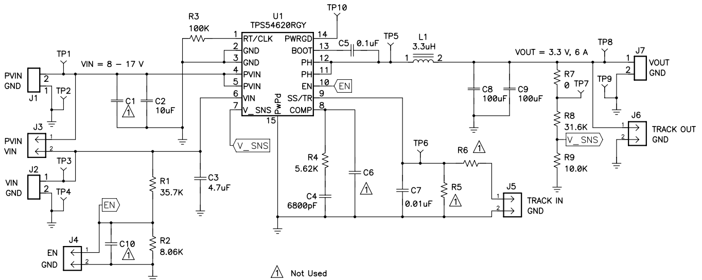
Figure 17. TPS54620EVM-374 Schematic
