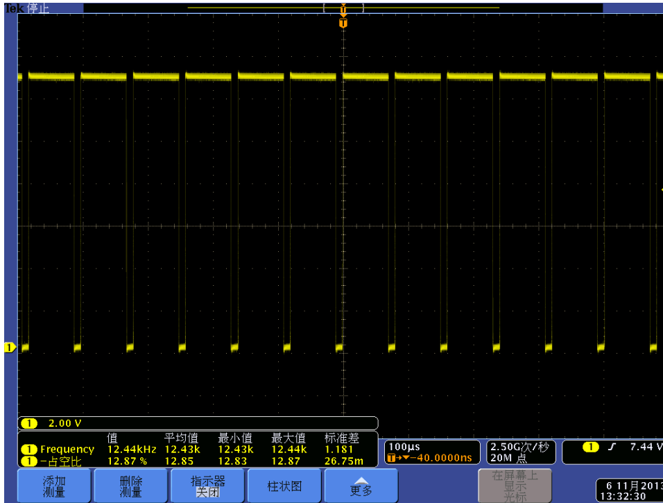
Fig 11, Output voltage – set to 12.5% PWM duty (12.5kHz)
