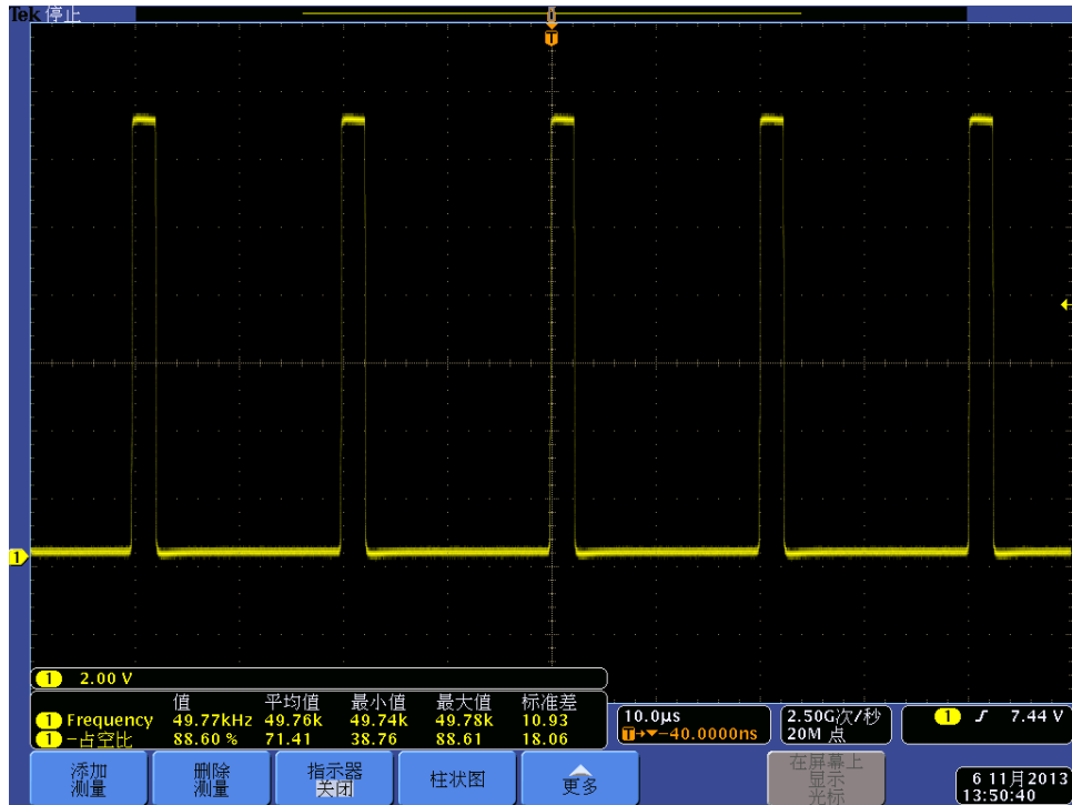
Fig 17, Output voltage – set to 87.5% PWM duty (50kHz)
