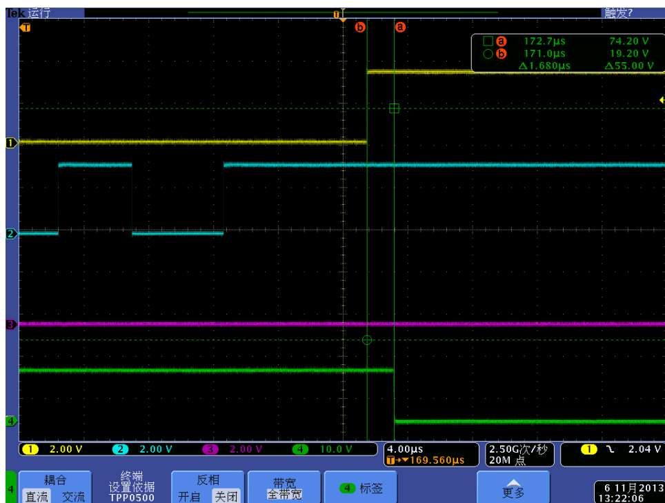
Fig 9, Delay between the rising edge of LATCH and outputs updated
