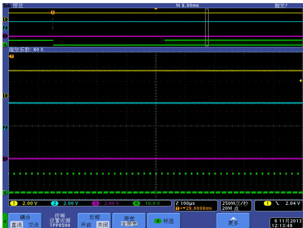
(Yellow: LATCH; Blue: CLK; Purple: DIN; Green: OUT4 of #1)
