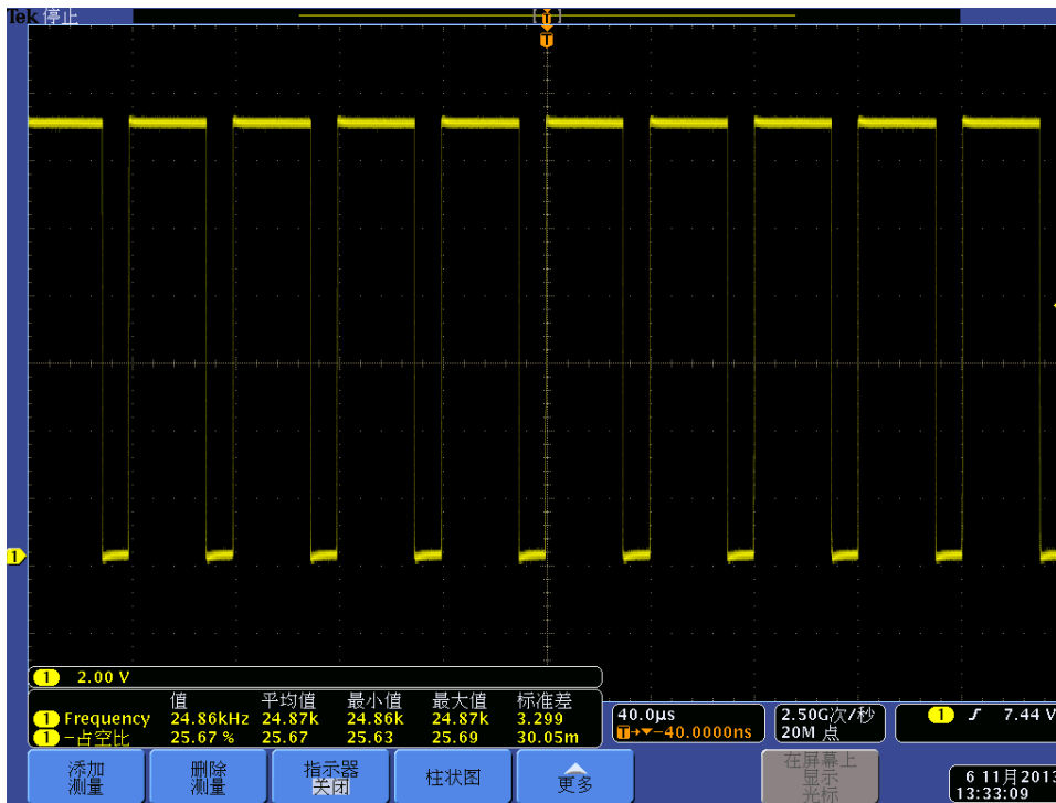
Fig 12, Output voltage – set to 25% PWM duty (25kHz)
