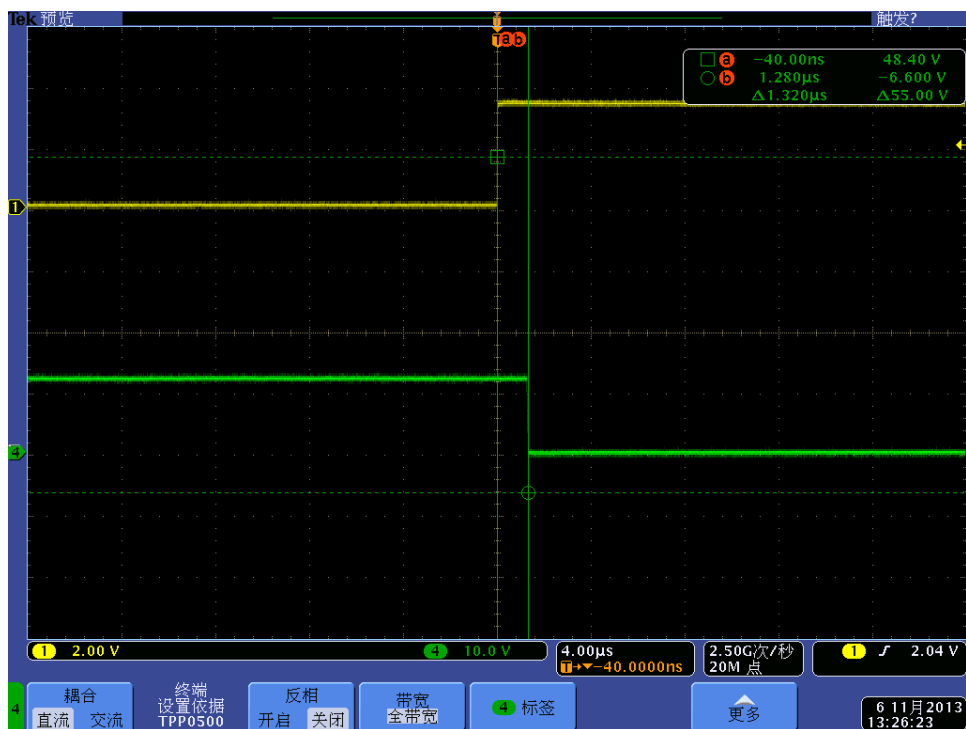
Fig 10, Delay between ENABLE and outputs ON
