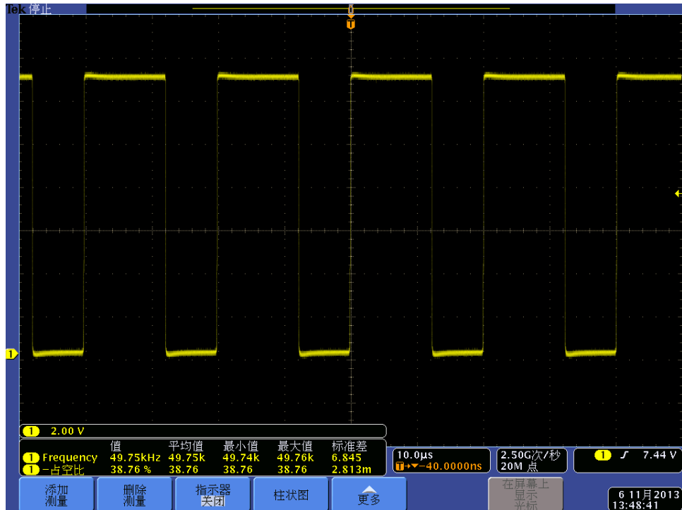
Fig 13, Output voltage – set to 37.5% PWM duty (50kHz)
