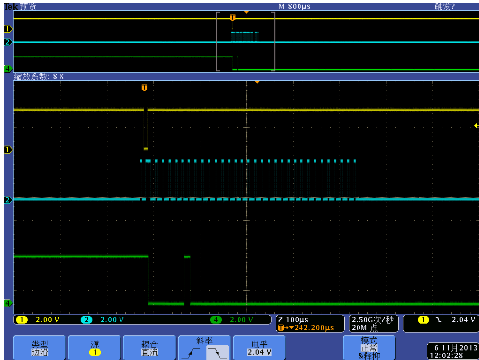
(Yellow: LATCH; Blue: CLK; Green: DOUT2) Fig 3, Example of read back OCP fault (Set outputs ON first).
