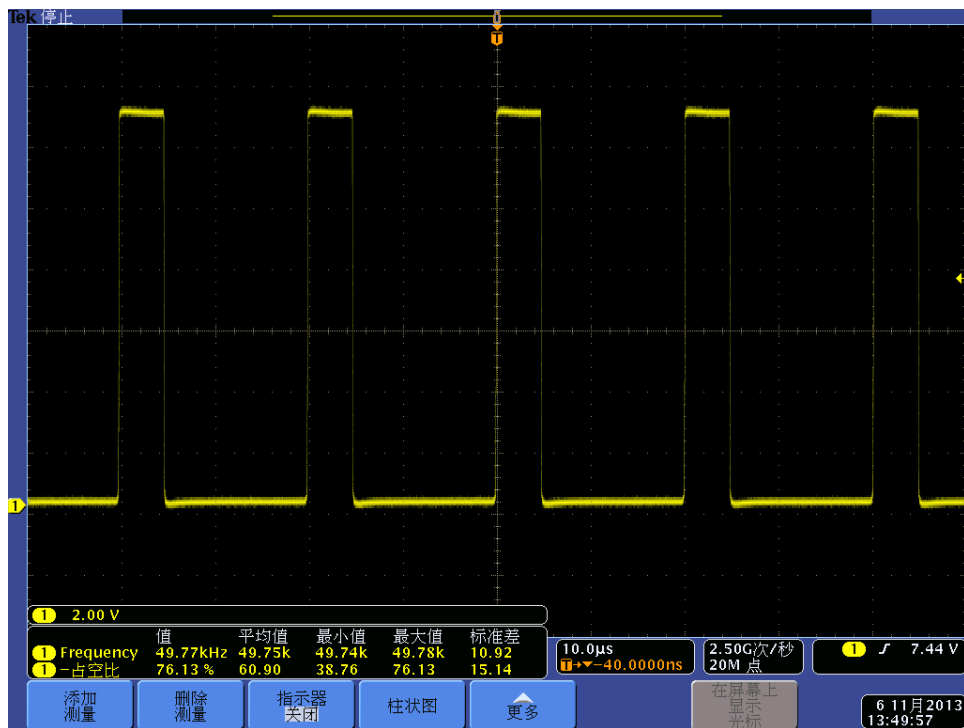
Fig 16, Output voltage – set to 75% PWM duty (50kHz)
