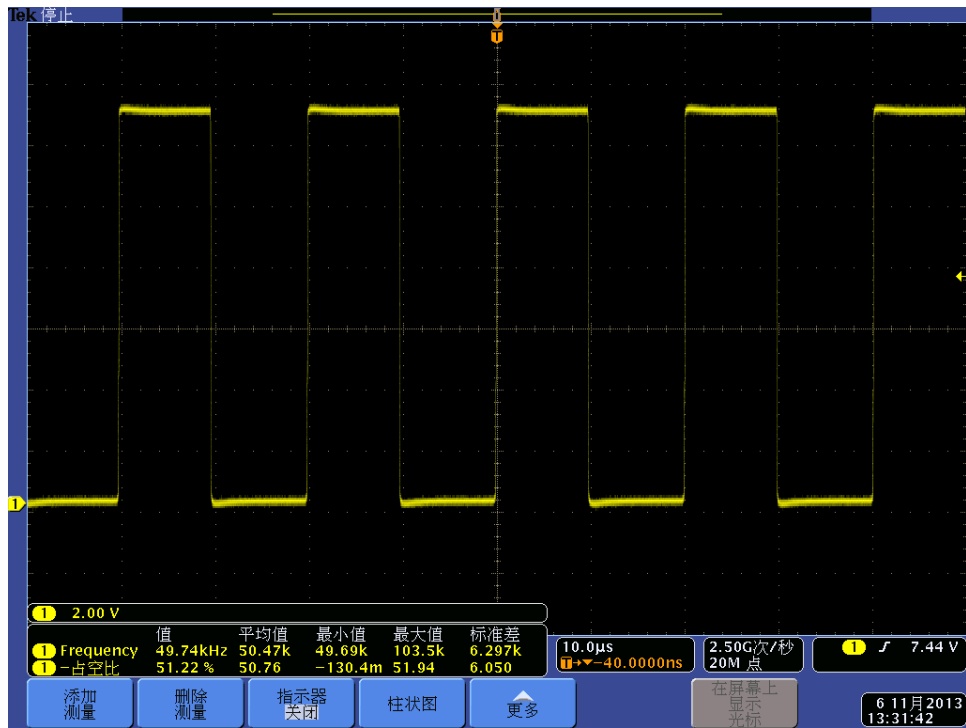
Fig 14, Output voltage – set to 50% PWM duty (50kHz)
