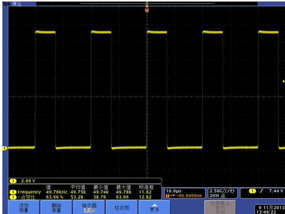
Fig 15, Output voltage – set to 62.5% PWM duty (50kHz)
