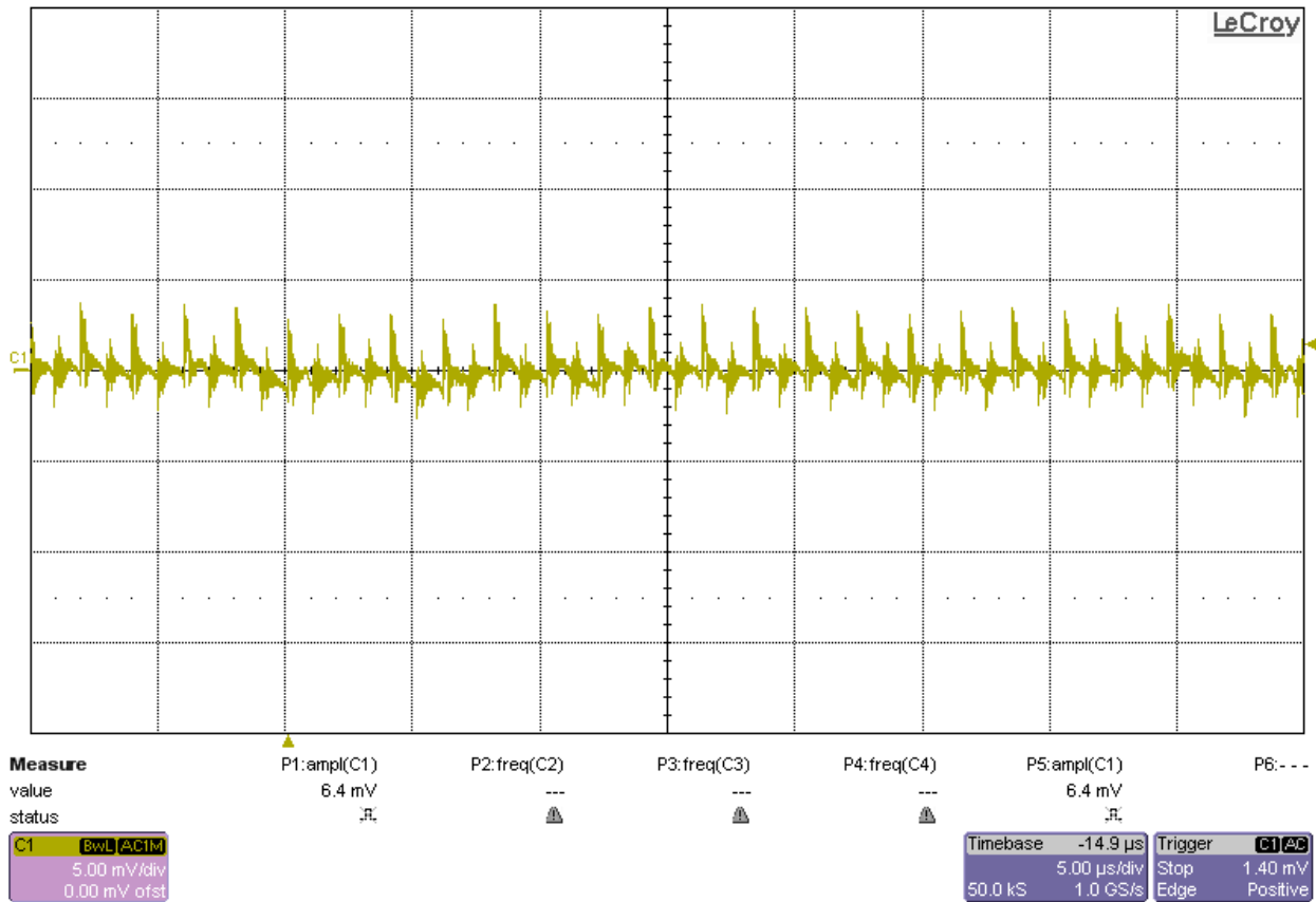
Figure 26. VIN = 12V, VCCINT Output Ripple @ IOOUT = 60A
