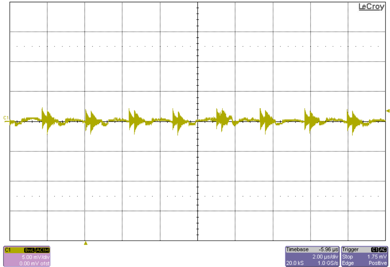
Figure 33. VIN = 12V, VCC1V2 Output Ripple @ IOU = 10A
