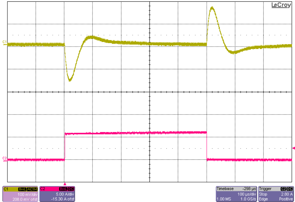
Figure 43. VIN = 12V, UTIL_12V Load Transient
