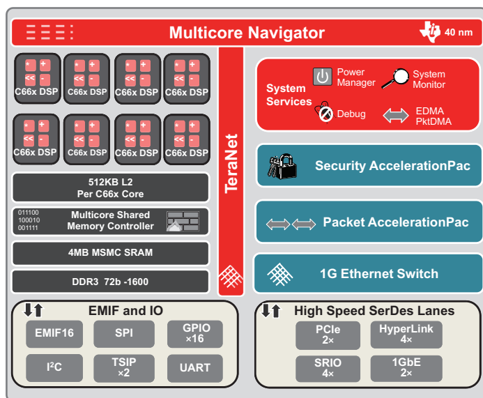
Figure 1: TMS320C6678 block diagram
