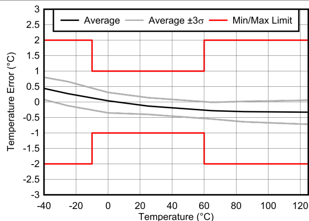
Figure 6-4. TMP1075NDR1 Temperature Error vs. Temperature
