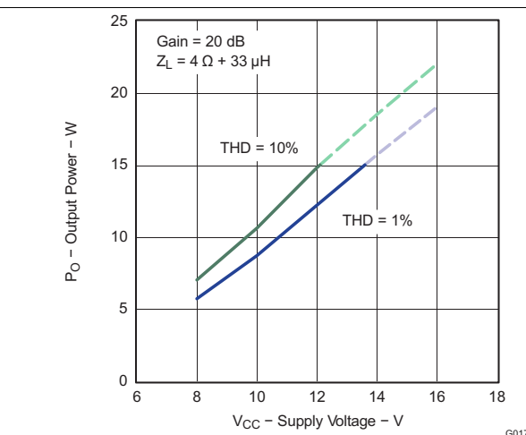
Note: Dashed Lines represent thermally limited regions. Figure 45. Output Power vs Supply Voltage (BTL)
