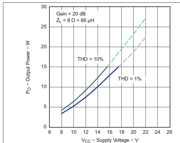
Note: Dashed Lines represent thermally limited regions. Figure 44. Output Power vs Supply Voltage (BTL)
