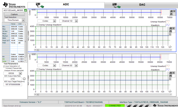
Figure 7-10. Idle-Channel Noise (No Input) for 2.5-GSPS, Dual-Channel Oscilloscope
