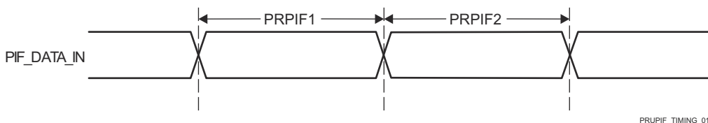
Figure 6-96. PRU_ICSSG PRU Peripheral Interface Timing Requirements
