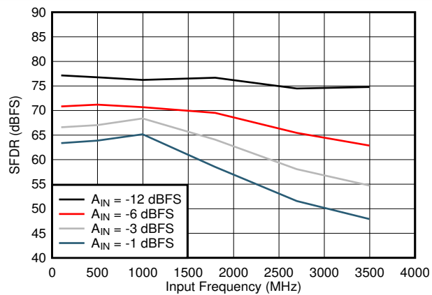
Figure 5-17. SFDR vs Input Frequency
