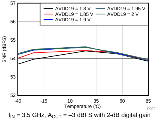
Figure 33. Signal-to-Noise Ratio vs AVDD19 Supply and Temperature
