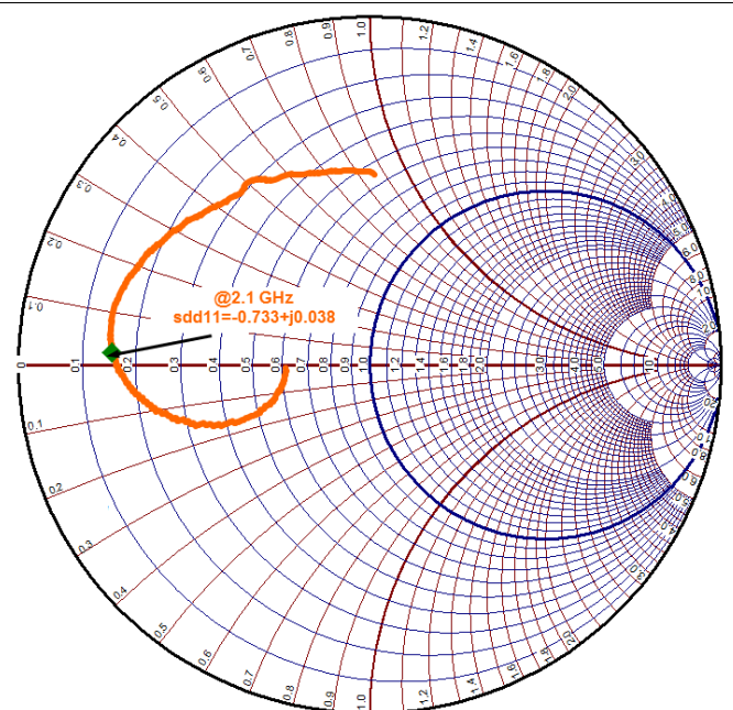
Figure 61. SDD11 Over the Input Frequency Range
