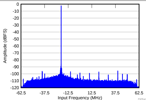
Figure 57. FFT in 24X Decimation (Complex Output)
