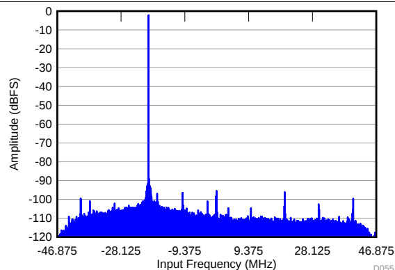
Figure 58. FFT in 32X Decimation (Complex Output)
