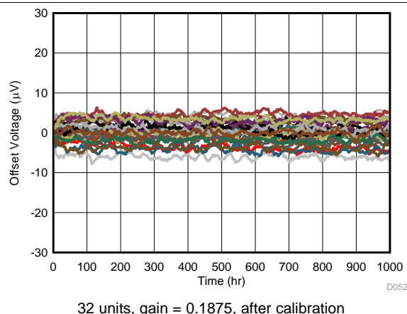
Figure 27. Offset Voltage Long-Term Drift
