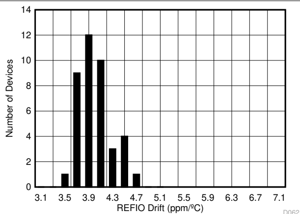
Figure 7-11. Internal Reference Temperature Drift Histogram
