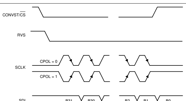
Figure 7-27. Standard SPI Timing Protocol (CPHA = 1, 32 SCLK Cycles)
