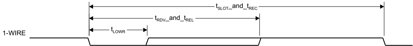
Figure 5-108. 1-Wire Read Bit Timing (Data)
