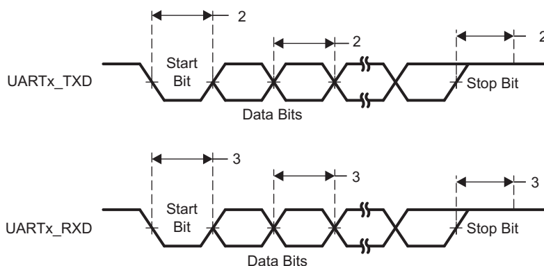
Figure 5-135. UART Timings
