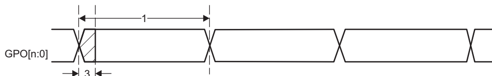
Figure 5-111. PRU-ICSS PRU Direct Output Timing
