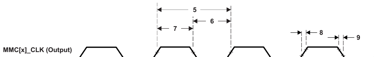
Figure 5-132. MMC[x]_CLK Timing
