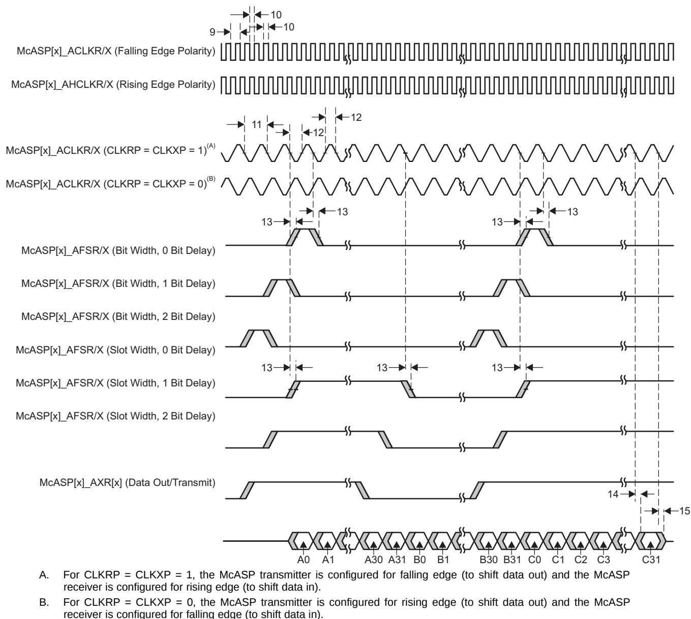
Figure 5-96. McASP Output Timing
