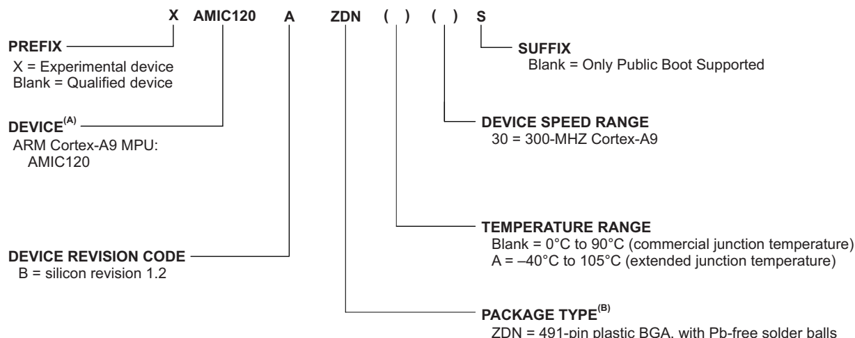
Figure 6-1. Device Nomenclature
