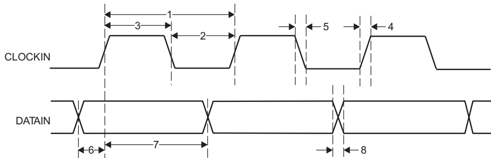
Figure 5-112. PRU-ICSS PRU Parallel Capture Timing - Rising Edge Mode
