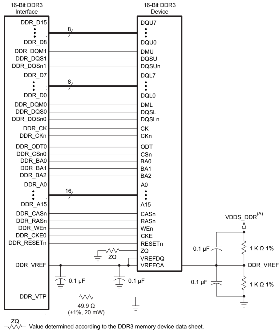
Figure 5-50. 16-Bit DDR3 Interface Using One 16-Bit DDR3 Device Without V_{\Pi} Termination
