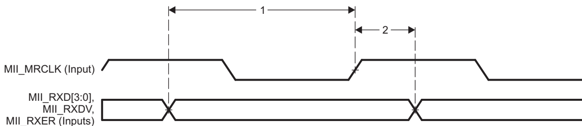
Figure 5-128. PRU-ICSS MII_RXD[3:0], MII_RXDV, and MII_RXER Timing
