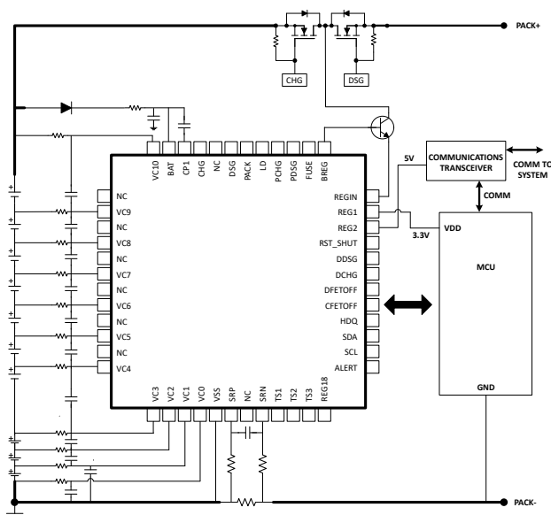
Simplified Schematic
