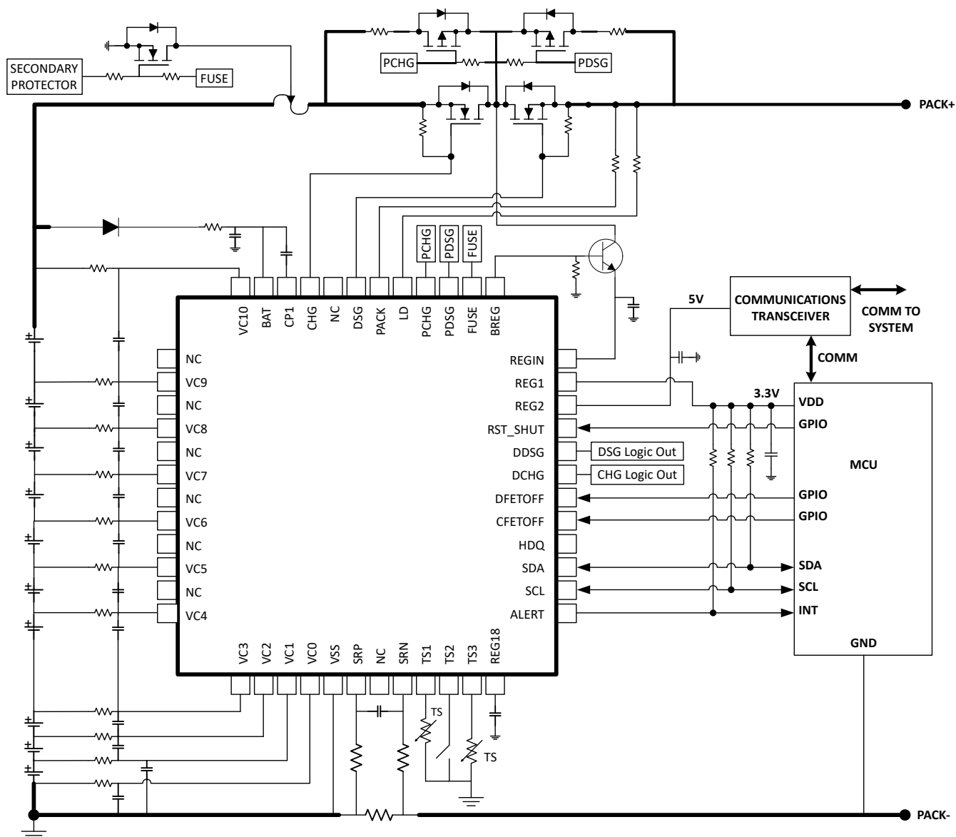
Figure 16-1. BQ76942 10-Series Cell Typical Implementation (Simplified Schematic)
