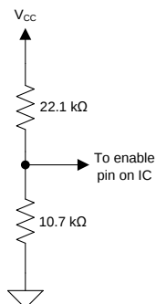
Figure 50. Voltage Divider Used to Hold Enable Low at Power-Up or Power-Down
