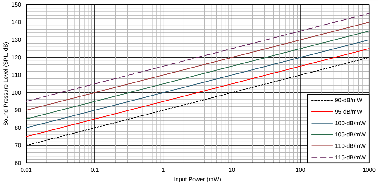
Figure 56. Sound Pressure Level vs Input Power for Headphones of Various Efficiencies
