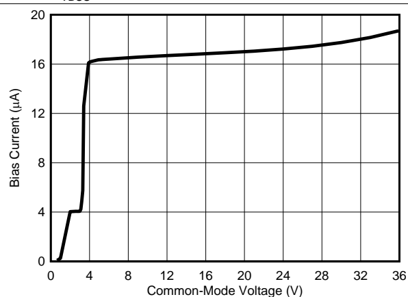
Figure 14. Input Bias Current vs Common-Mode Voltage (Both Inputs, IN+ and IN-)
