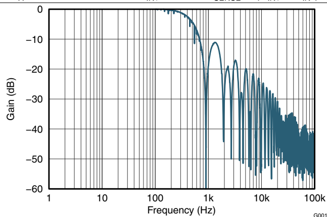
Figure 13. Frequency Response
