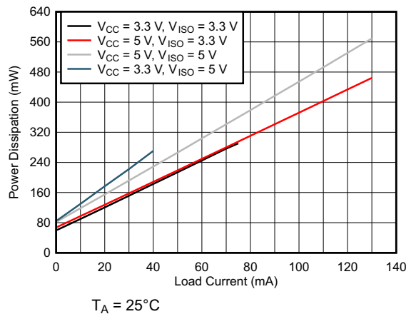
Figure 7-7. ISOW7841 Power Dissipation vs Load Current ( I_{ISO} )
