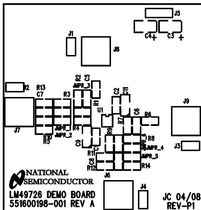
Figure 49. Top Silkscreen
