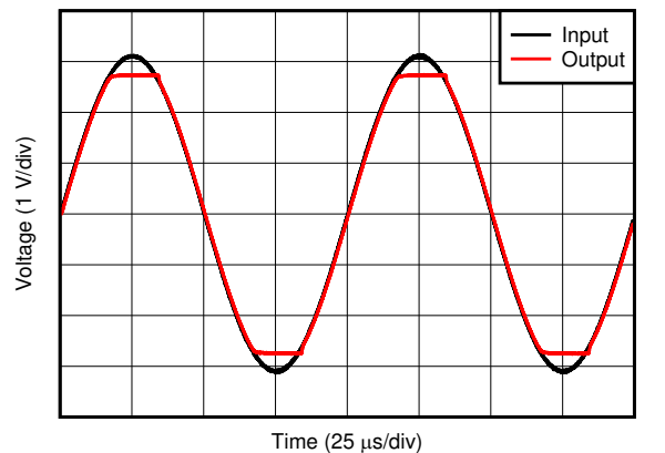
Figure 7-29. No Phase Reversal
