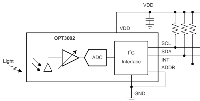
Block Diagram
