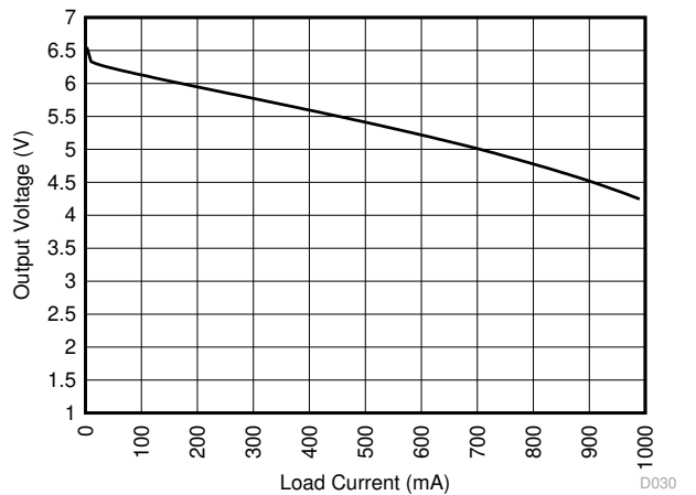
Figure 6-3. Output Voltage vs Load Current
