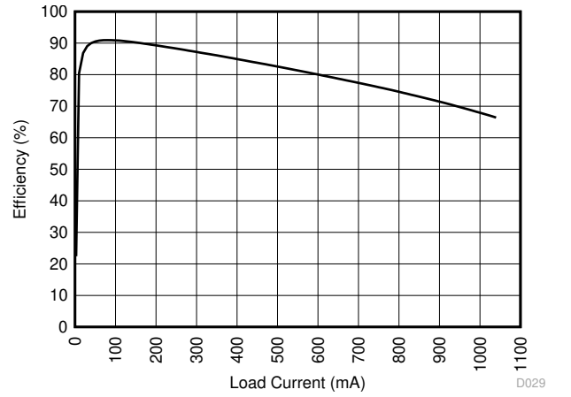
Figure 6-2. Efficiency vs Load Current
