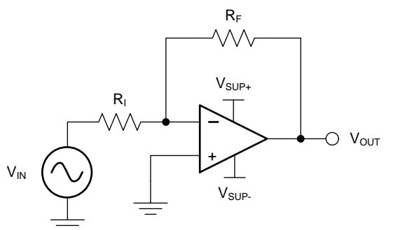
Figure 15. Application Schematic
