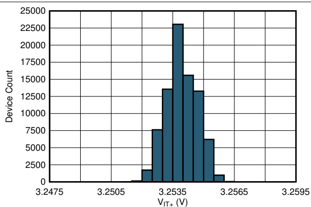
Figure 7-14. Positive Threshold Histogram
