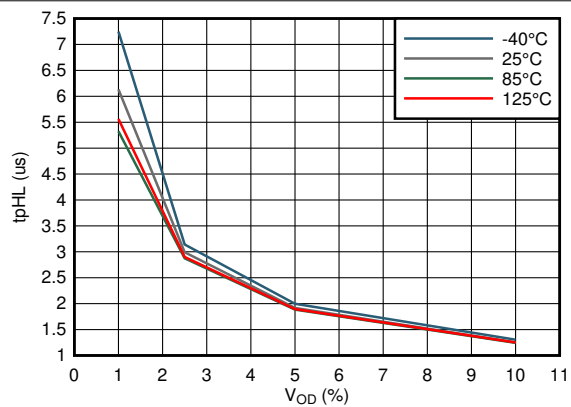
Figure 7-31. Propagation Delay High-Low vs Input Overdrive
