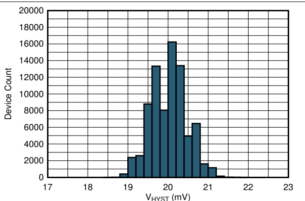
Figure 7-6. Hysteresis Histogram
