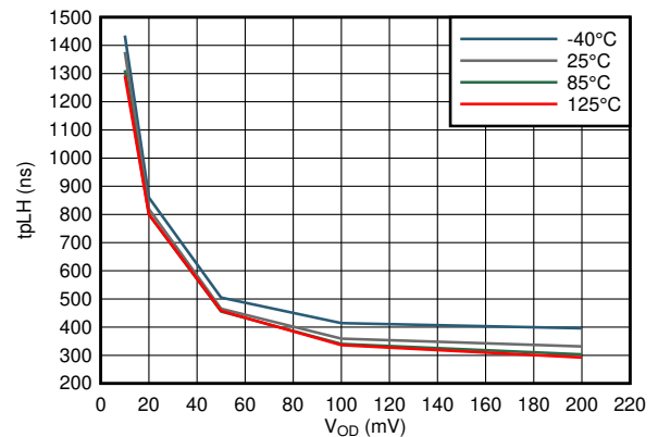
Figure 7-28. Propagation Delay Low-High vs Input Overdrive TLV40x1R2
