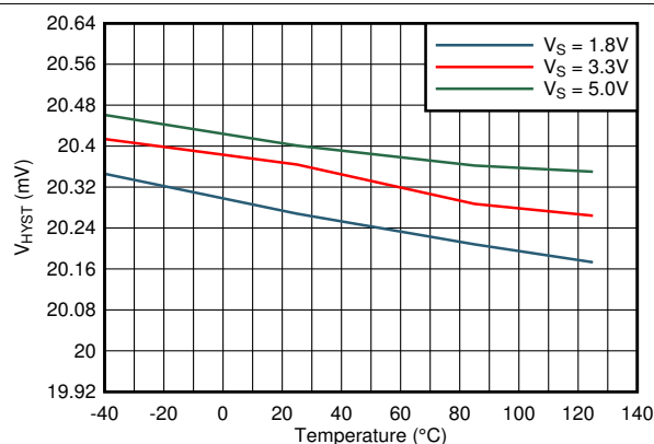
Figure 7-5. Hysteresis vs Temperature
