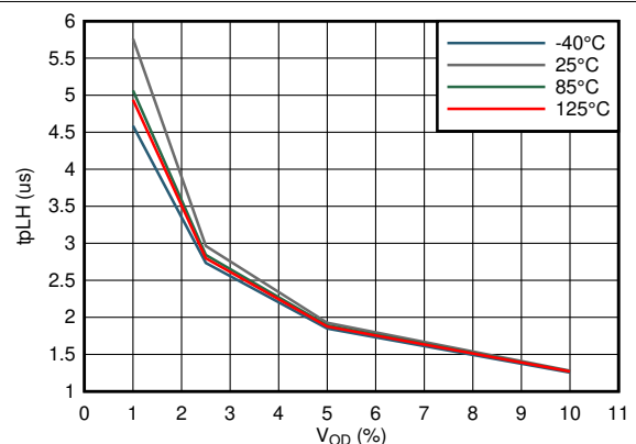
Figure 7-30. Propagation Delay Low-High vs Input Overdrive TLV4021Sx5
