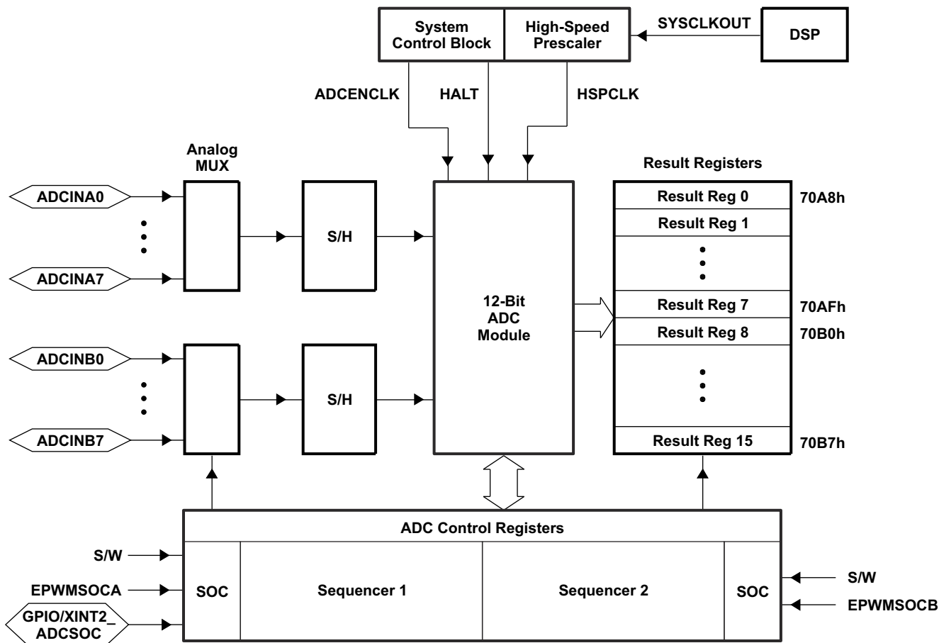
Figure 9-7. Block Diagram of the ADC Module
