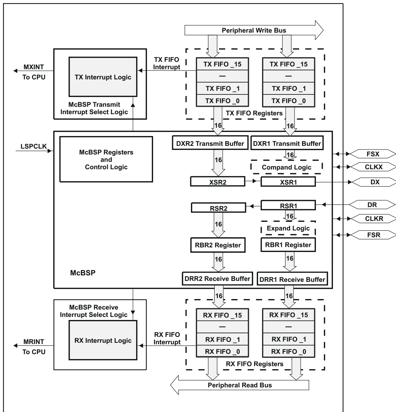
Figure 9-9. McBSP Module With FIFO
