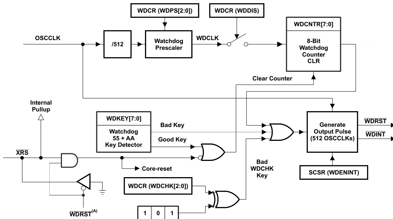
Figure 9-22. Watchdog Module
