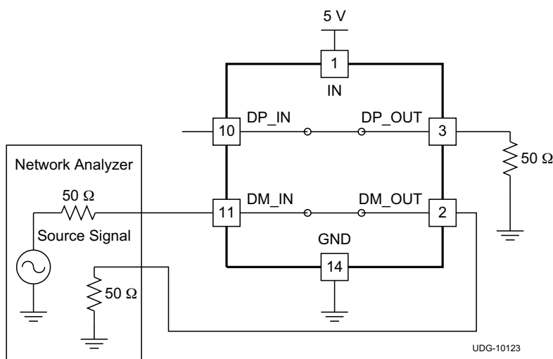
Figure 38. Bandwidth (BW)
