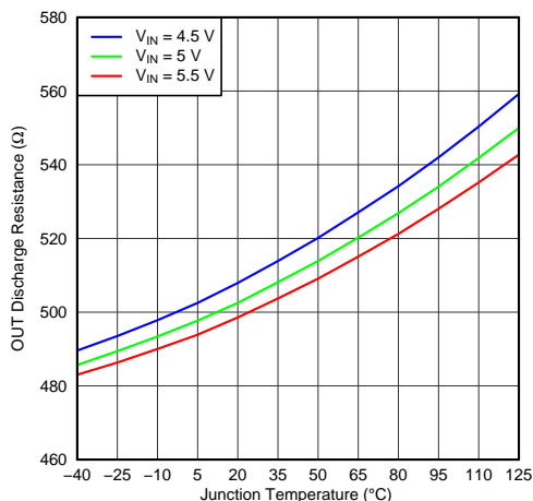
Figure 3. OUT Discharge Resistance vs Temperature
