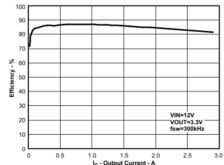
Figure 57. Efficiency vs Load Current
