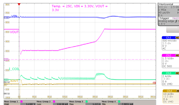
Figure 8-38. Start-up with 100-mA ICL
