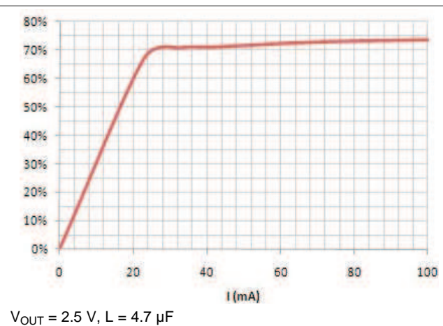
Figure 4. BUCK2 Efficiency
