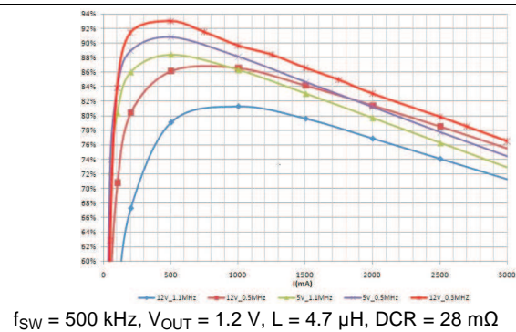
Figure 2. BUCK1 Efficiency
