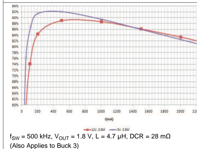
Figure 5. BUCK2 Efficiency
