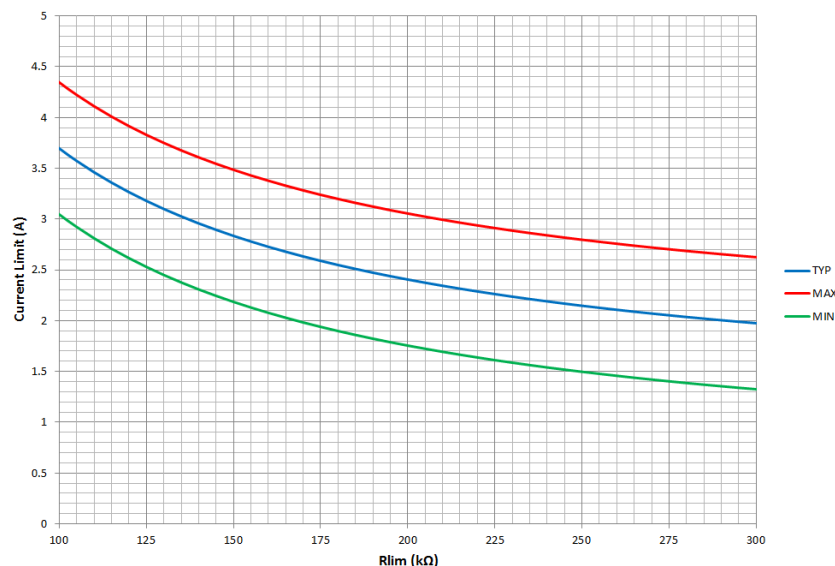
Figure 19. Buck 3
