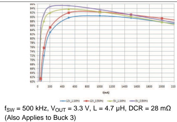
Figure 4. BUCK2 Efficiency
