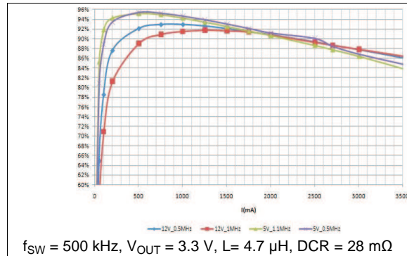
Figure 1. BUCK1 Efficiency
