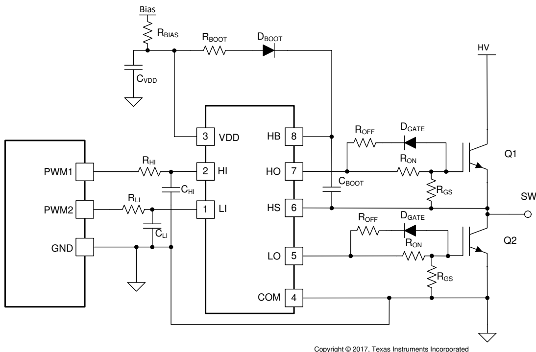
Figure 46. Typical IGBT Application Schematic
