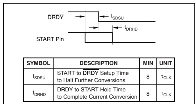
Figure 42. START Pin and \overline{DRDY} Timing
