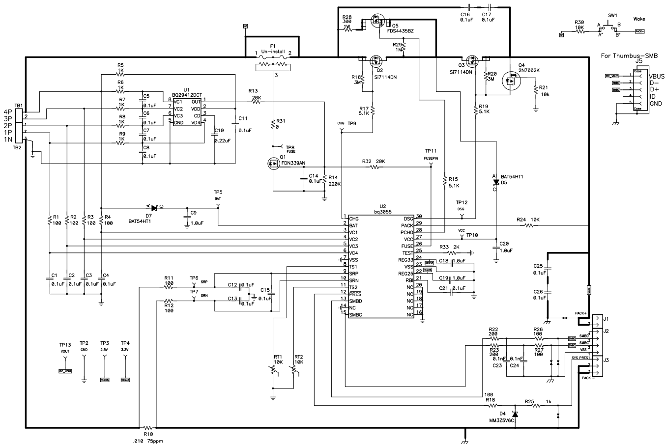
Figure 6. Application Schematic
