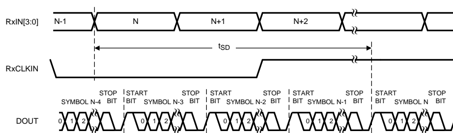
Figure 6. Latency Delay
