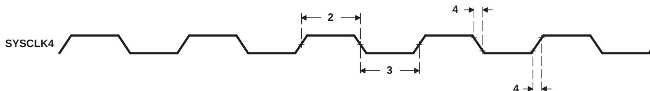
Figure 7-22. SYSCLK4 Timing
