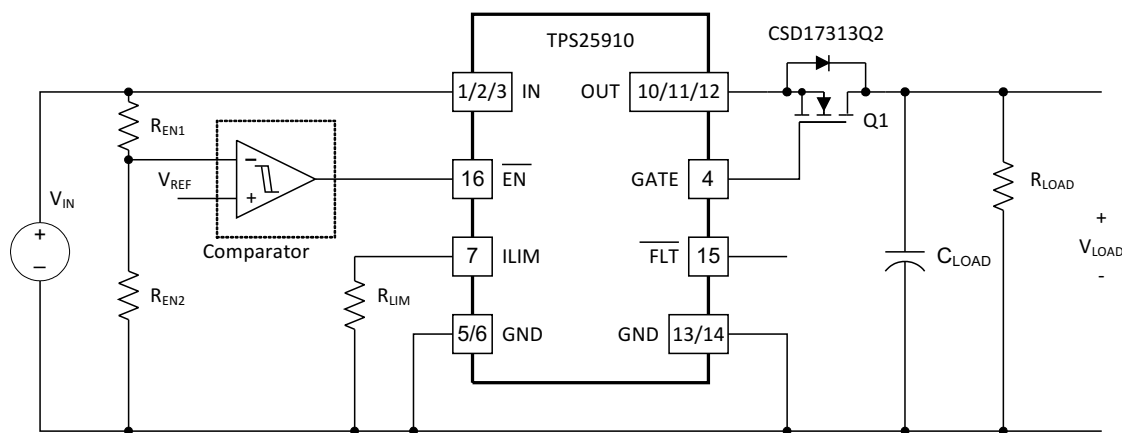
Figure 10. B2B Implementation
