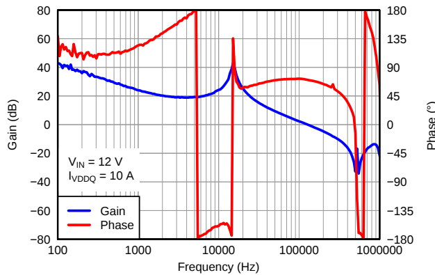
Figure 30. VDDQ Bode Plot
