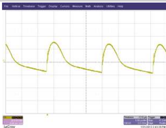
Figure 46. Ripple with 5-V, 1.2-A Output, 265-V AC Input, 20 mV/div 5 \mu s/div
