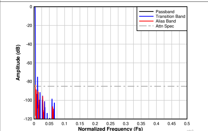
Figure 7-35. Complex Decimation by 128 Filter Response
