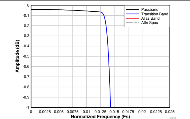
Figure 7-31. Decimation by 32 Passband Ripple Response
