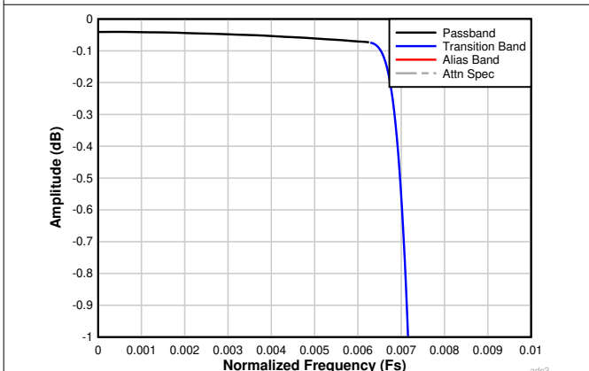
Figure 7-34. Decimation by 64 Passband Ripple Response
