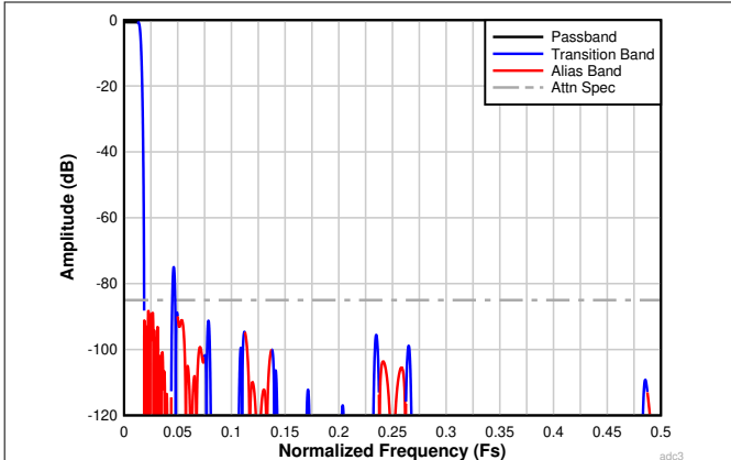
Figure 7-30. Complex Decimation by 32 Filter Response
