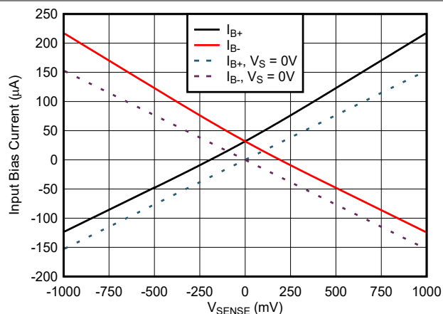
Figure 6-19. INA241x2-Q1 Input Bias Current vs V_{\text{SENSE}}
