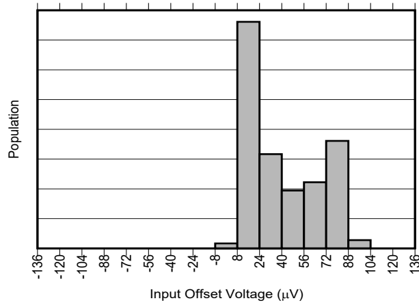
Figure 6-5. All Gains INA241B-Q1 Input Offset Production Distribution
