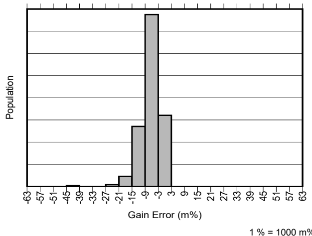
Figure 6-12. All Gains INA241B-Q1 Gain Error Production Distribution
