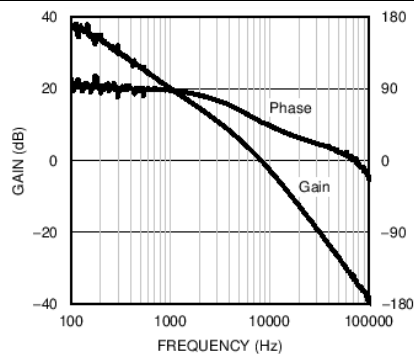
Figure 25. Overall Loop Gain and Phase - Buck Mode
