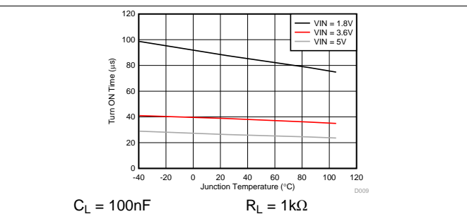
Figure 8. Turn ON Time vs Junction Temperature
