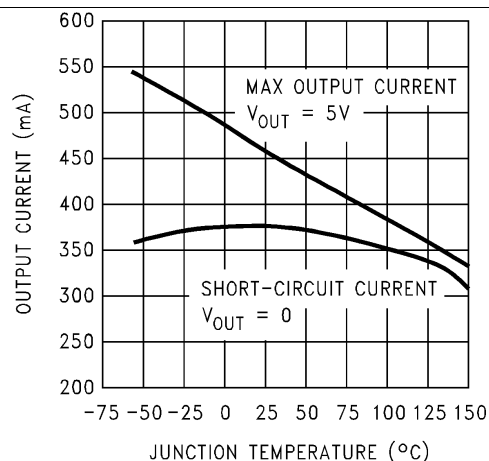
Figure 18. Short-Circuit Output Current and Maximum Output Current
