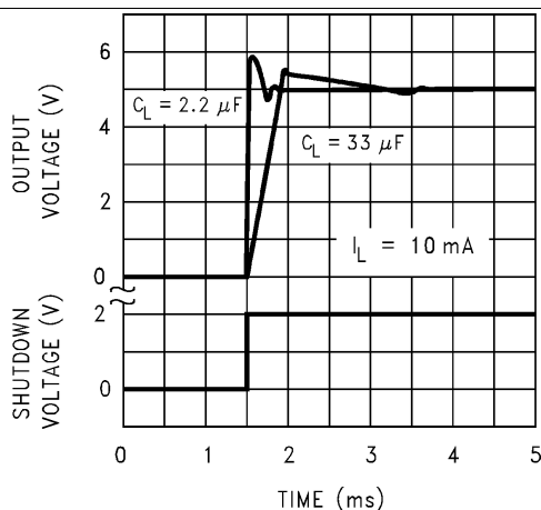
Figure 17. Enable Transient
