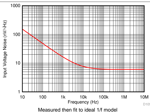
Figure 49. Input Voltage Noise Density vs Frequency
