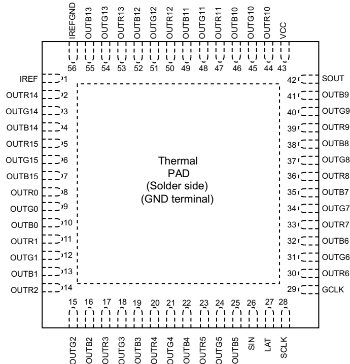
Pin Functions
