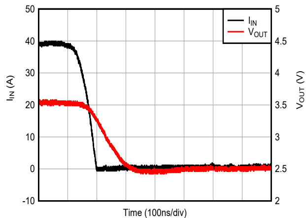
Figure 6-12. Voltage Output Step Response, Falling
