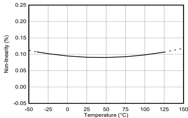
Figure 6-5. Non-Linearity vs Temperature
