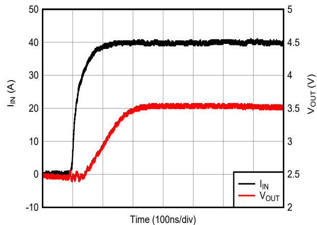
Figure 6-11. Voltage Output Step Response, Rising
