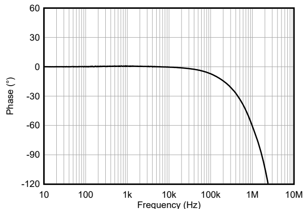
Figure 6-8. Phase vs Frequency, All Gains
