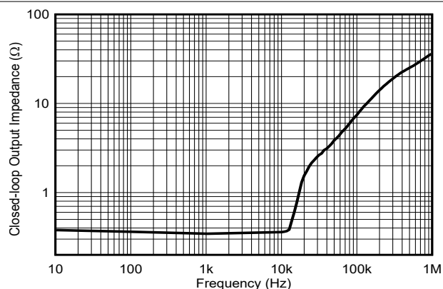
Figure 6-10. Output Impedance vs Frequency
