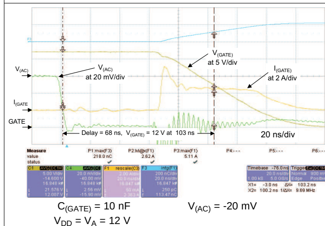
Figure 19. Turnoff Time
